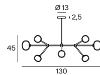
552.10L Chandelier
