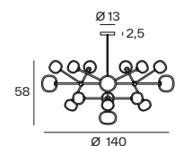
552.16L Chandelier
