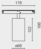
LED ARRAY Up to 20W
