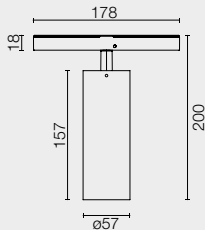
LED ARRAY 22,5W
