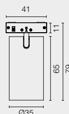
LIGHT STRIPE WALL-WASHER
