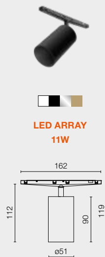
LIGHT SHADOW SPOT 45
