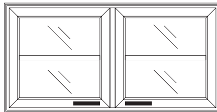
3048/A Pensile 2P Wall unit L 128 P 37 H 65
