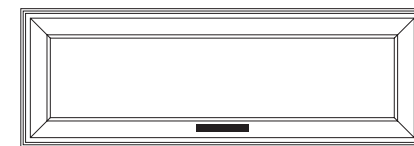
3049/A Pensile 1 p. apertura frontale Wall unit front opening L 120 P 37 H 40
