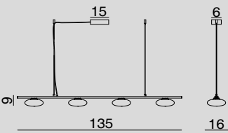
1713.135.4L SOSPENSIONE A ROSONE / HANGING LAMP WITH CANOPY Glass 4 x Ø 16 cm - Cable 200 cm 4 x LED 7.5W DIMM
