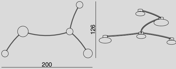
COS1726.5L PLAFONIERA / CEILING LAMP Glass 3 x Ø16, 1 x Ø21, 1 x Ø25 cm 5 x LED 7.5W DIMM
