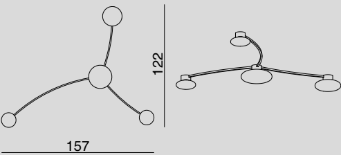
COS1726.4L PLAFONIERA / CEILING LAMP Glass 2 x Ø16, 1 x Ø21, 1 x Ø25 cm 4 x LED 7.5W DIMM
