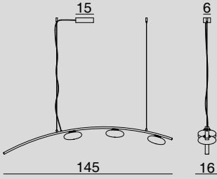
1703.150.3L SOSPENSIONE A ROSONE / HANGING LAMP WITH CANOPY Glass 3 x Ø 16 cm - Cable 200 cm 3 x LED 7.5W DIMM
