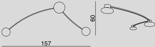
COS1726.3L PLAFONIERA / CEILING LAMP Glass 2 x Ø16, 1 x Ø21 cm 3 x LED 7.5W DIMM
