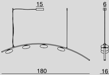
1703.180.4L SOSPENSIONE A ROSONE / HANGING LAMP WITH CANOPY Glass 4 x Ø 16 cm - Cable 200 cm 4 x LED 7.5W DIMM
