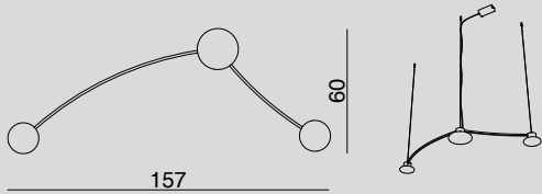
COS1723.3L SOSPENSIONE A ROSONE / HANGING LAMP WITH CANOPY Glass 2 x Ø16, 1 x Ø21 cm - Cable 200 cm 3 x LED 7.5W DIMM
