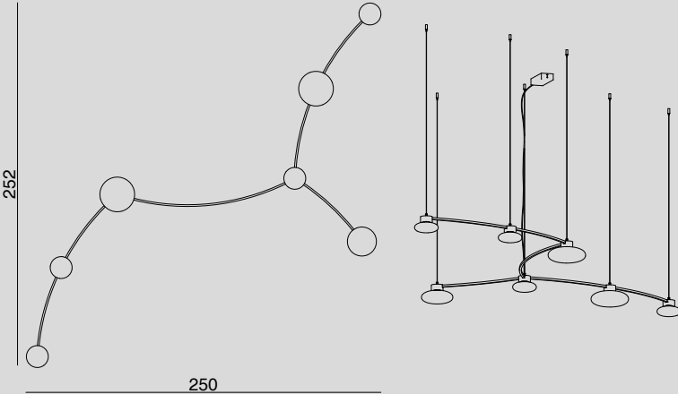
COS1723.7L SOSPENSIONE A ROSONE / HANGING LAMP WITH CANOPY Glass 4 x Ø16, 1 x Ø21, 2 x Ø25 cm - Cable 200 cm 7 x LED 7.5W DIMM
