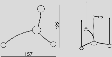
COS1723.4L SOSPENSIONE A ROSONE / HANGING LAMP WITH CANOPY Glass 2 x Ø16, 1 x Ø21, 1 x Ø25 cm - Cable 200 cm 4 x LED 7.5W DIMM
