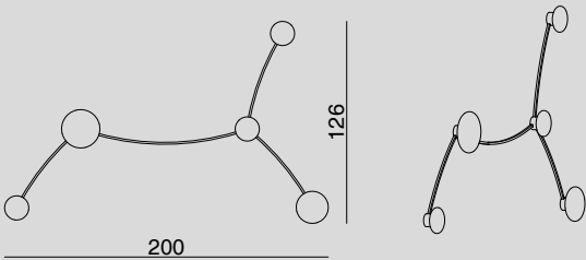
COS1721.5L APPLIQUE / WALL LAMP Glass 3 x Ø16, 1 x Ø21, 1 x Ø25 cm 5 x LED 7.5W DIMM
