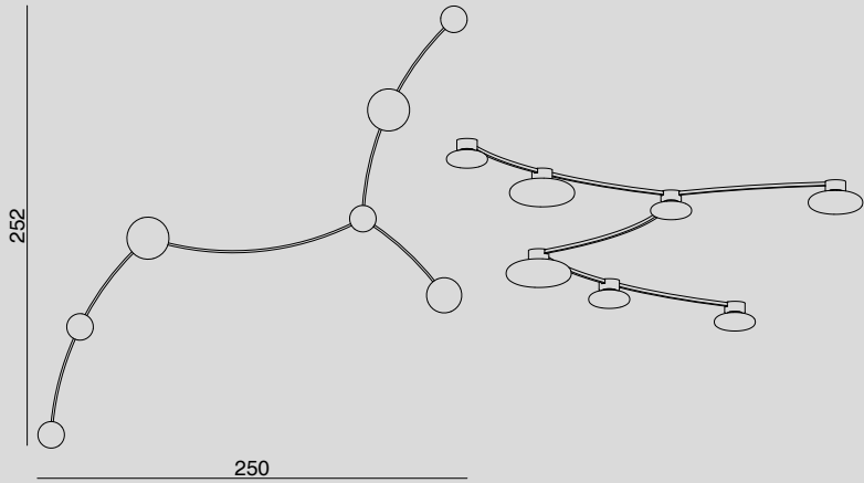
COS1726.7L PLAFONIERA / CEILING LAMP Glass 4 x Ø16, 1 x Ø21, 2 x Ø25 cm 7 x LED 7.5W DIMM
