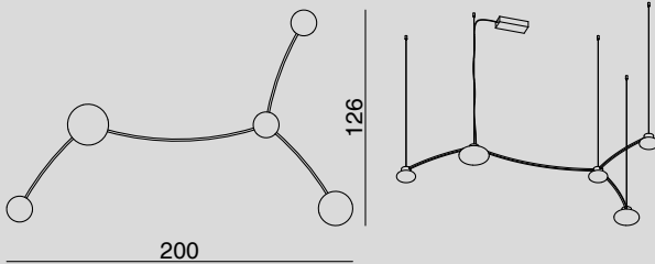
COS1723.5L SOSPENSIONE A ROSONE / HANGING LAMP WITH CANOPY Glass 3 x Ø16, 1 x Ø21, 1 x Ø25 cm - Cable 200 cm 5 x LED 7.5W DIMM
