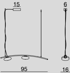
1703.90.2L SOSPENSIONE A ROSONE / HANGING LAMP WITH CANOPY Glass 2 x Ø 16 cm - Cable 200 cm 2 x LED 7.5W DIMM
