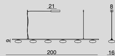
1713.200.6L SOSPENSIONE A ROSONE / HANGING LAMP WITH CANOPY Glass 6 x Ø 16 cm - Cable 200 cm 6 x LED 7.5W DIMM
