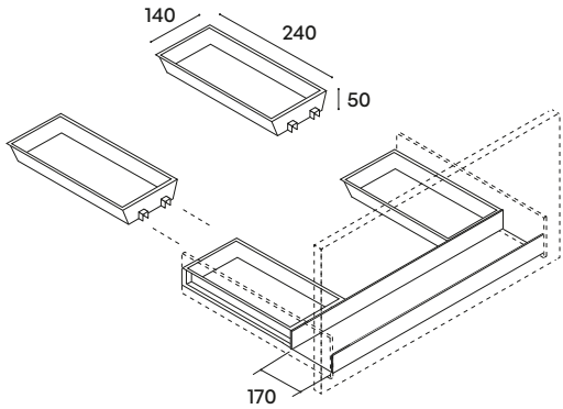
. Vaschette sottolavello kit 2 vaschette ad incastro Under sink trays kit 2 interlocking trays
