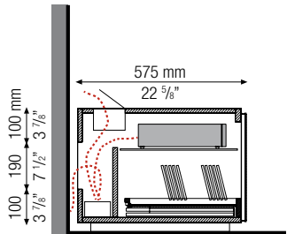
scatola passacavi / cables flap box
