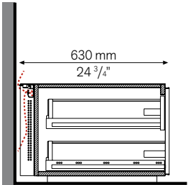
canalina passacavi / cables flap trough
