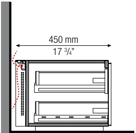
canalina passacavi / cables flap trough
