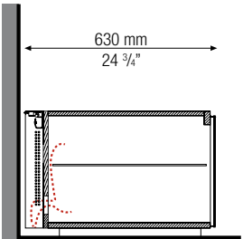
passacavi / cables flap
