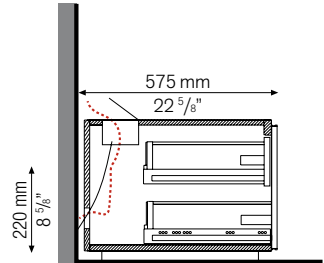
passacavi + scatola passacavi / cables flap + cables flap box
