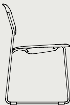
SOFT EDGE 50/55 SEAT UPH. W50 x D52,5 x H79/SH47,5 cm
