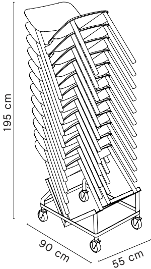
Soft Edge 60 Max. 12 pcs. H195 x W55 x D90 cm Stacking is not possible with seat upholstery
