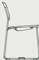
SOFT EDGE 52/56 SEAT UPH. W. HOOK LINK W52,5 x D52,5 x H79/SH47,5 cm
