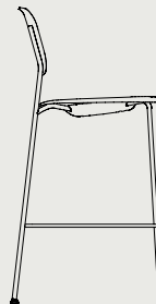
SOFT EDGE 90/95 HIGH SEAT UPH. W55 x D55,5 x H108/SH75 cm
