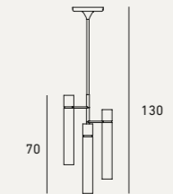
3 Identical Elements-Ø7
