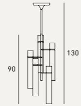
5 Identical Elements-Ø7
