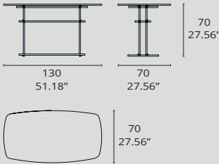
4230/81 V1 MESA | TABLE
