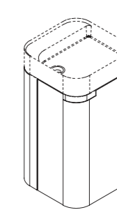
Free standing units Mobili freestanding W 45 X D 45 X H 88,5 cm
